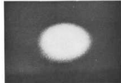
FIG. 2. (d). THE CLOUD OF JULY 5, 1964, IN Sr I LIGHT AS SEEN FROM LA MADDALINA 52 sec, 4 min, AND 22 min AFTER EVAPORATION.
